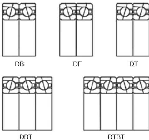
Fig.1.1 Duplex arrangement codes
