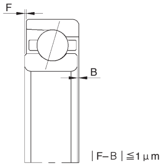
Fig.1.4 Flush grinding
